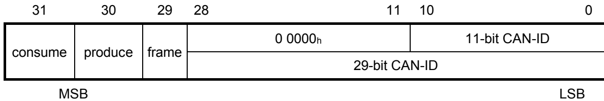
Figure 60: Structure of TIME COB-ID
