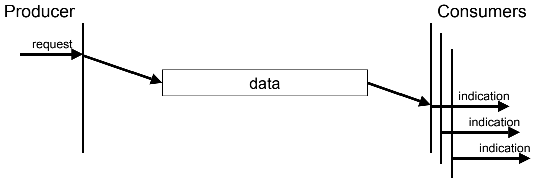
Figure 9: Push model
