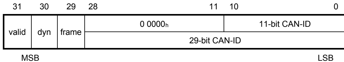
Figure 65: Structure of SDO server COB-ID
