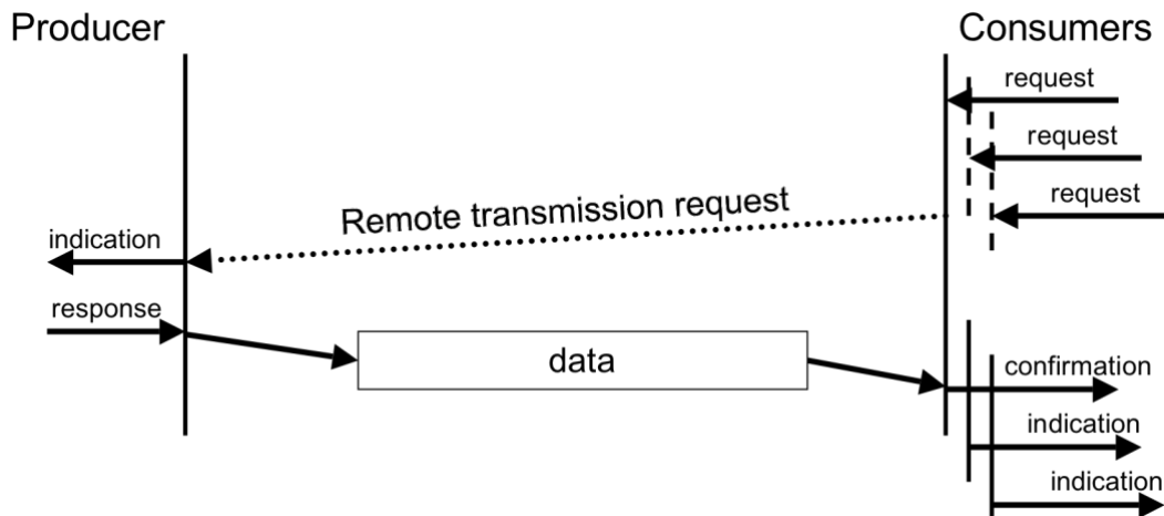
Figure 10: Pull model
