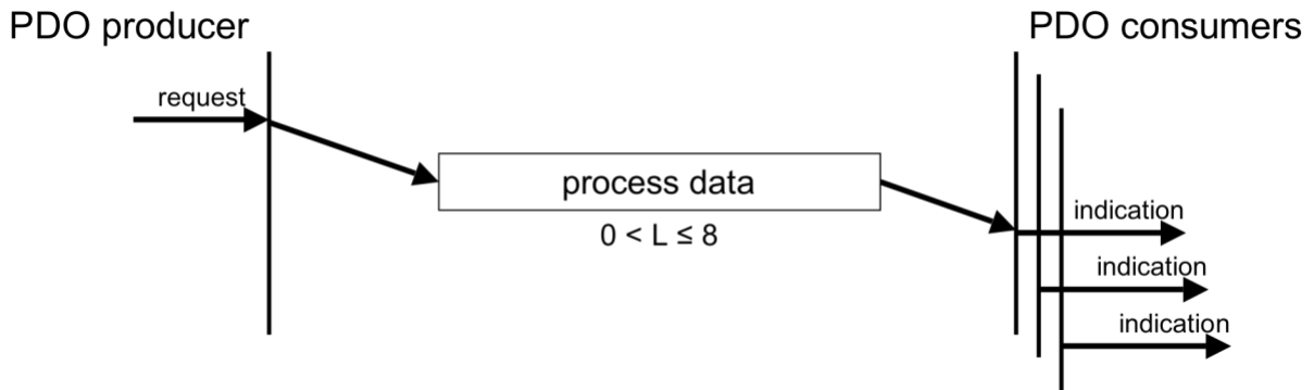
Figure 17: Protocol PDO write
