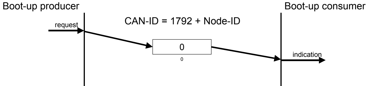
Figure 46: Protocol boot-up
